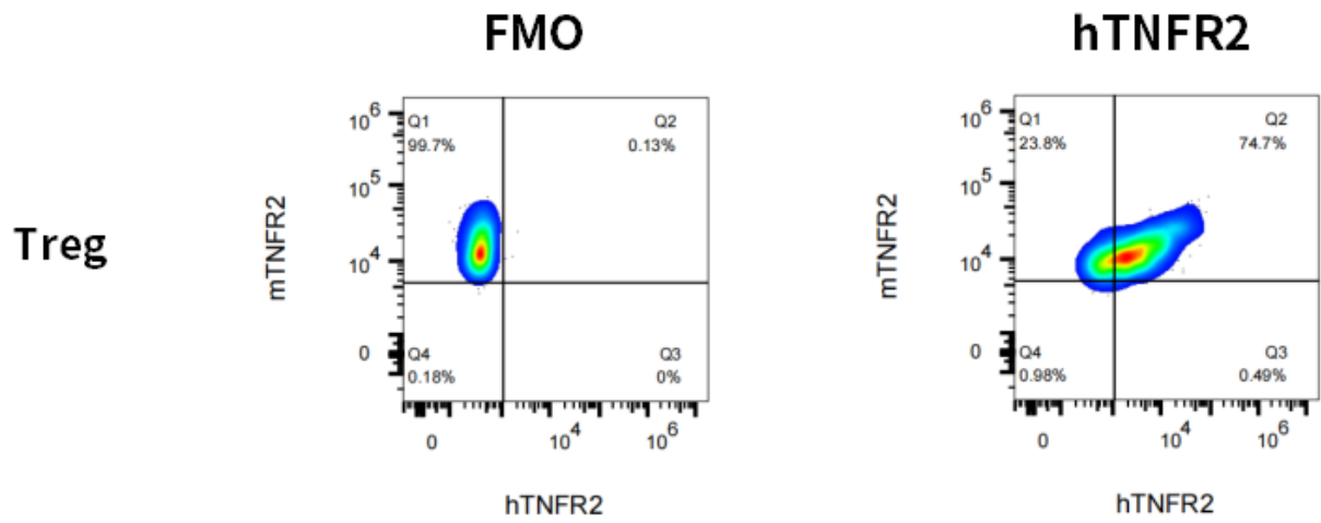
Fig.1 Expression characterization of hTNFR2 on Tregs in Spleen in heterozygous hTNFR2 KI mice.
